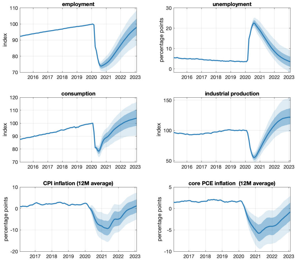
Figure 6: Baseline scenario: Forecasts of the impact of the Covid shock when the VAR is estimated using data from 1959:1. The solid lines represent actual data until April 2020, and posterior medians of the predictive density afterwards. The shaded areas correspond to 68- and 95-percent posterior credible regions.
