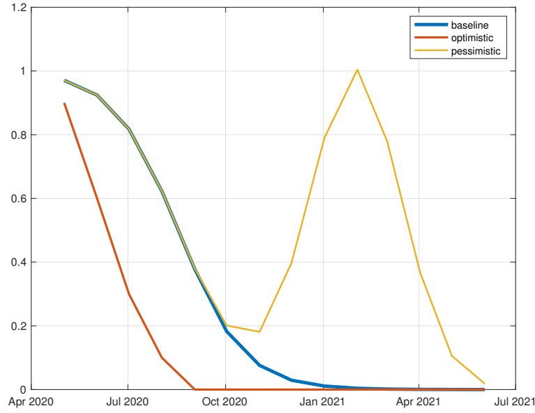
Figure 1: Pandemic scenarios, relative to April 2020.
