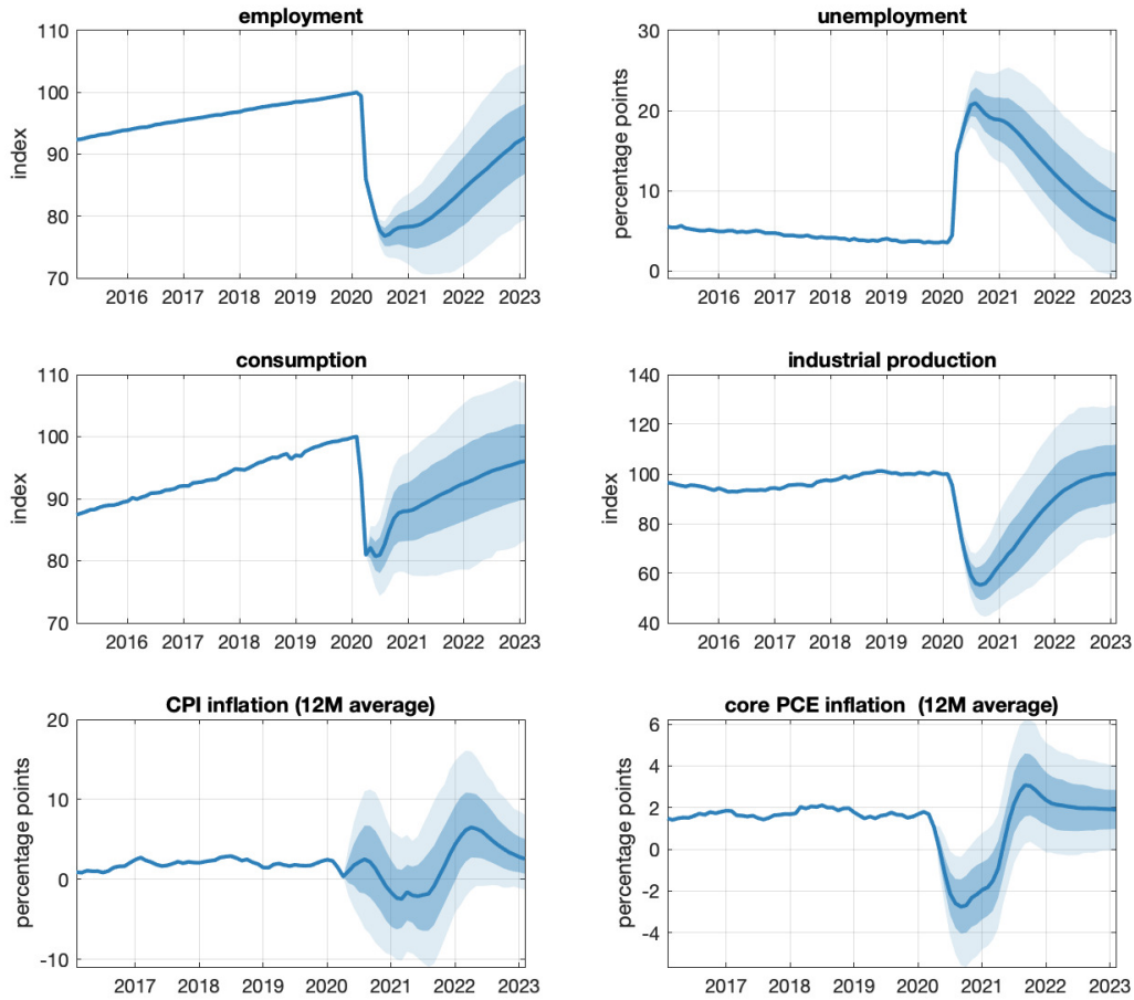
Figure 2: Baseline scenario: Forecasts of the impact of the Covid shock. The solid lines represent actual data until April 2020, and posterior medians of the predictive density afterwards. The shaded areas correspond to 68- and 95-percent posterior credible regions.
