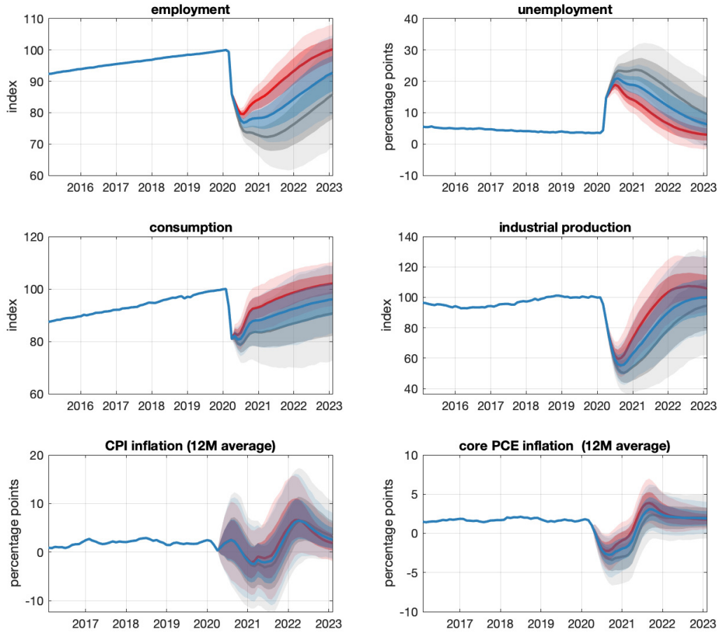
Figure 5: Baseline scenario: Forecasts of the impact of the Covid shock under three different assumptions about the external dynamics of shocks in normal times. The solid lines represent actual data until April 2020, and posterior medians of the predictive density afterwards. The shaded areas correspond to 68- and 95-percent posterior credible regions.
