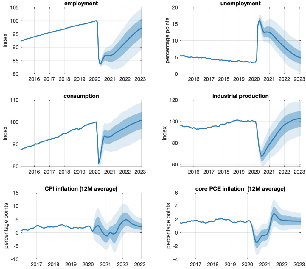
Figure 3: Optimistic scenario: Forecasts of the impact of the Covid shock. The solid lines represent actual data until April 2020, and posterior medians of the predictive density afterwards. The shaded areas correspond to 68- and 95-percent posterior credible regions.
