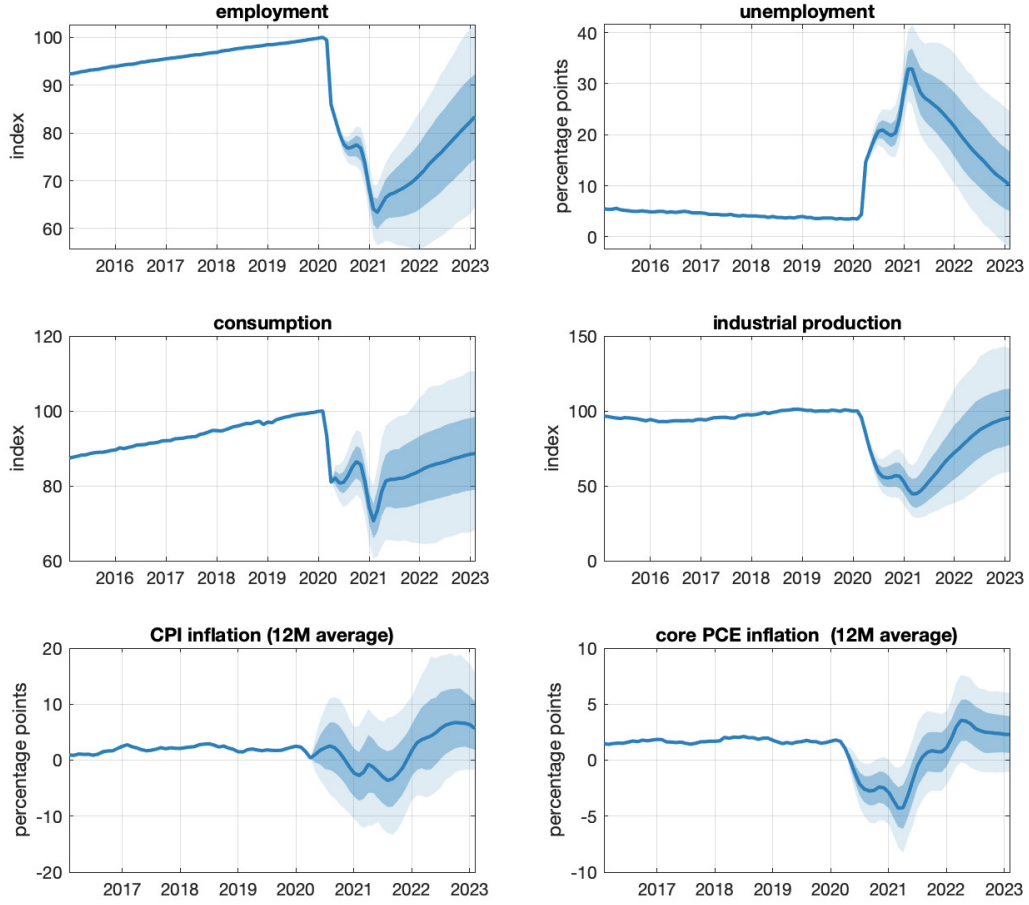
Figure 4: Pessimistic scenario: Forecasts of the impact of the Covid shock. The solid lines represent actual data until April 2020, and posterior medians of the predictive density afterwards. The shaded areas correspond to 68- and 95-percent posterior credible regions.
