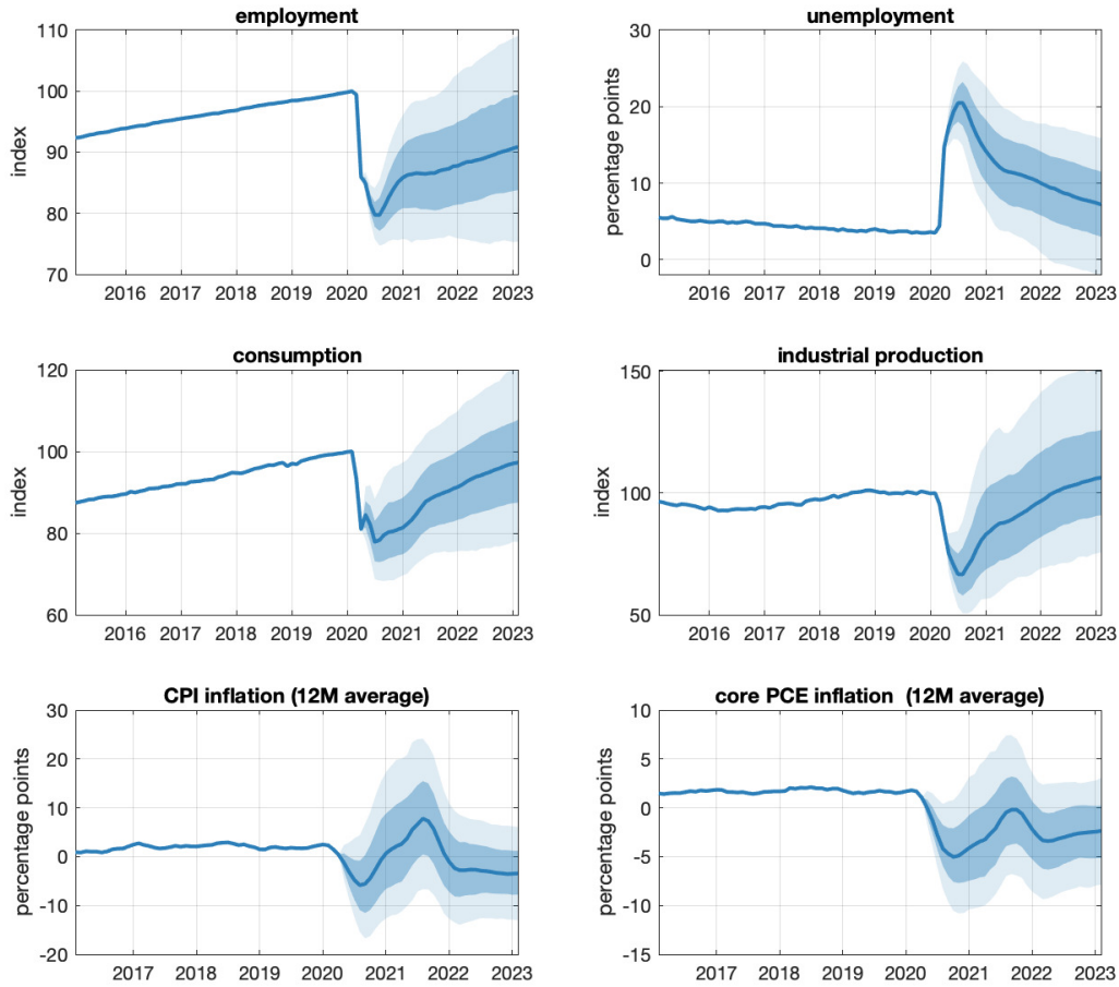
Figure 9: Baseline scenario: Forecasts of the impact of the Covid shock when the VAR is augmented with employment sectoral data. The solid lines represent actual data until April 2020, and posterior medians of the predictive density afterwards. The shaded areas correspond to 68- and 95-percent posterior credible regions.
